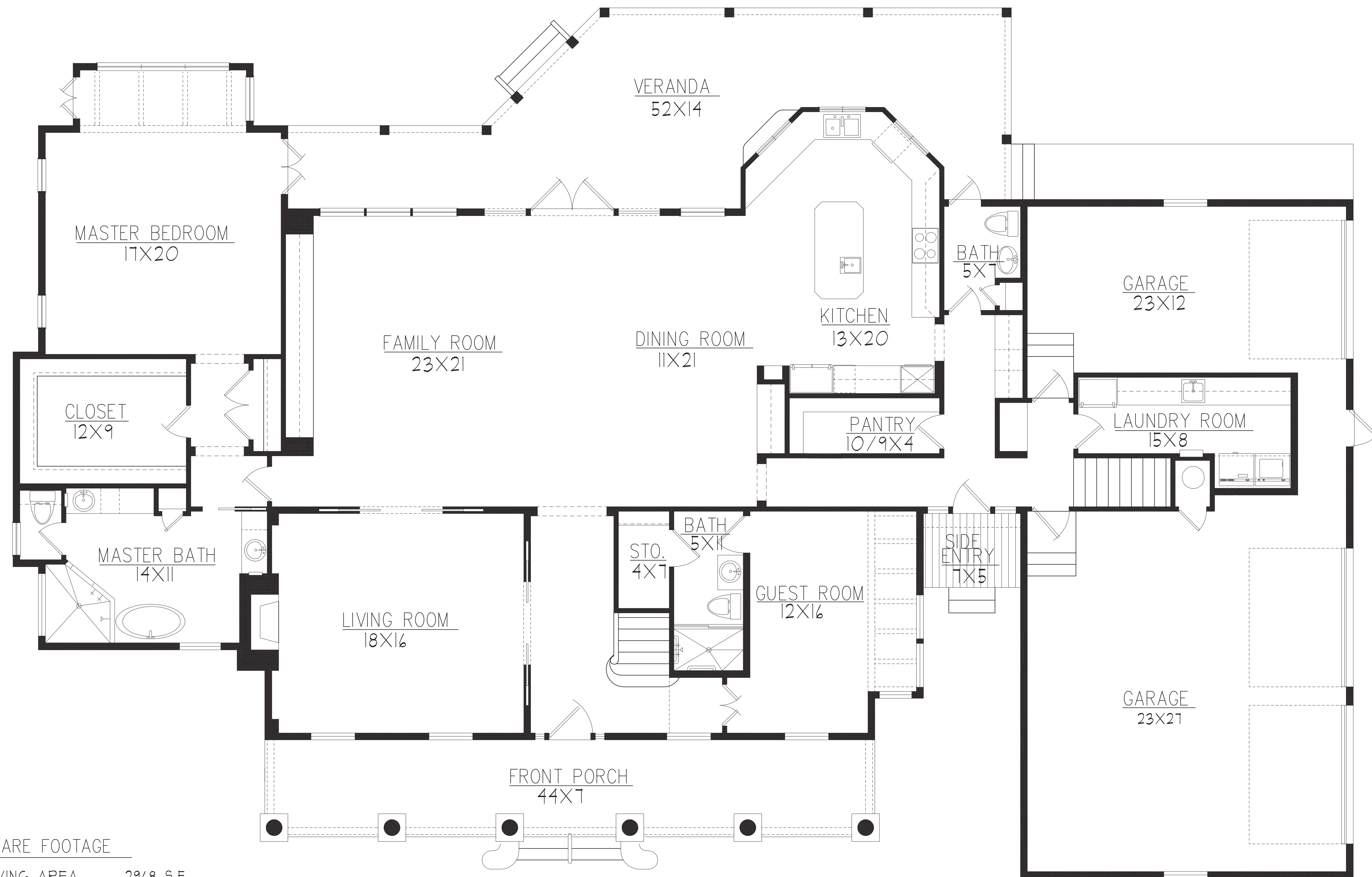
MAIN LEVEL FLOOR PLAN
